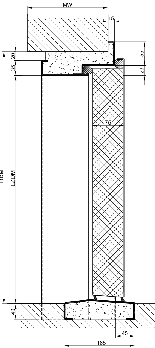
hump sill
