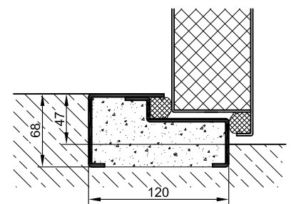
full sill
